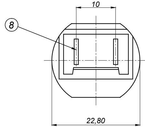
A - VIEW (TERMINAL DETAILS)
