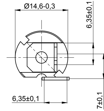
A - VIEW (TERMINAL DETAILS)
